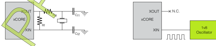
Figure 10: Example circuits using a crystal (left), or external oscillator (right).
