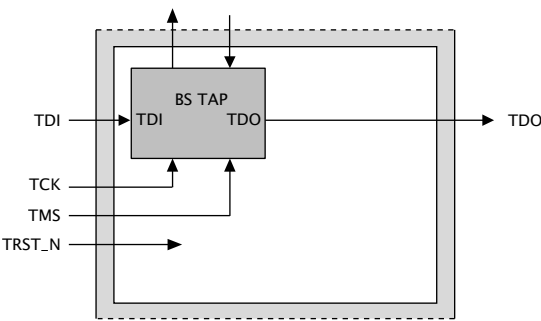
Figure 15: JTAG chain structure
